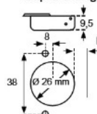
Cup drawing
